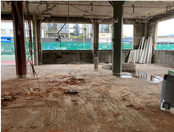
Broadway-City Hall, April 2021. Progressing with non-structural demolition.
