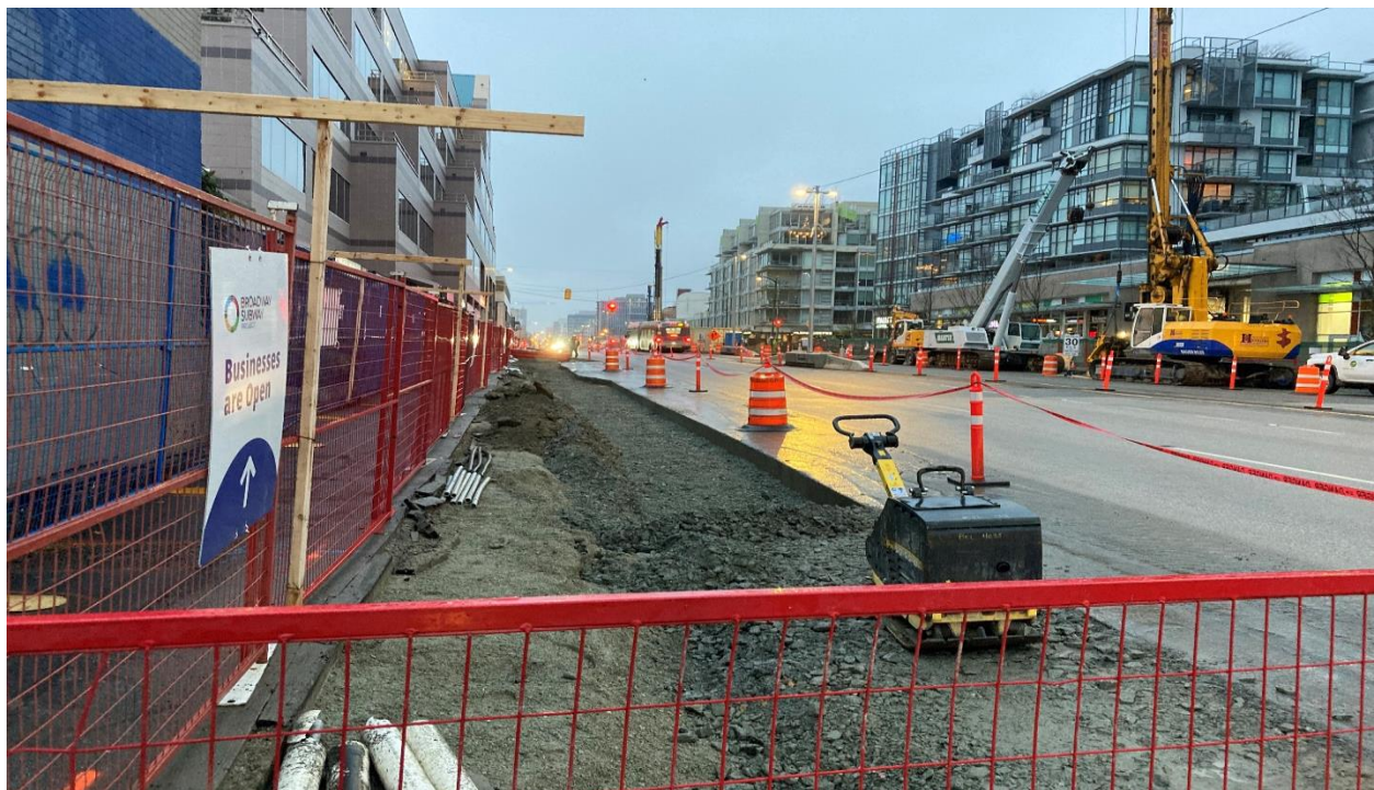
Figure 6: Arbutus Station: Progressing with the relocation of underground utilities and the installation of piles for the traffic decking.
