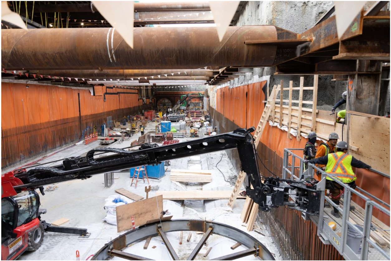
Figure 6: South Granville Station: Progressing with the installation of rebar and the rings in the headwalls.
