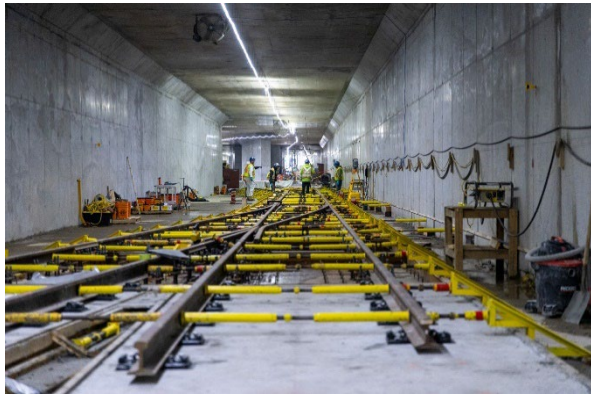
Figure 7: Arbutus Station: Progressing with aligning the track and pouring the concrete track base in the crossover section.
