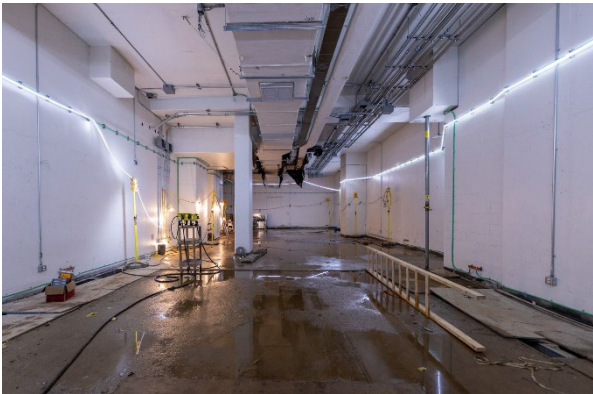
Figure 3: Mount Pleasant Station: Progressing with fit-out of the Propulsion Power Substation room.
