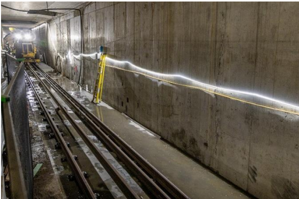
Figure 3: Mount Pleasant Station: Progressing with track installation in the inbound tunnel.
