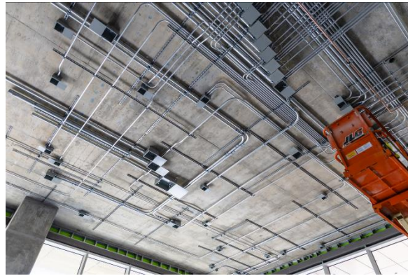
Figure 6: South Granville Station: Progressing with installation of electrical conduit in the station entrance.
