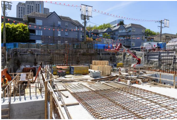
Figure 5: Oak-VGH Station: Progressing with rebar installation for the above-ground headhouse walls.
