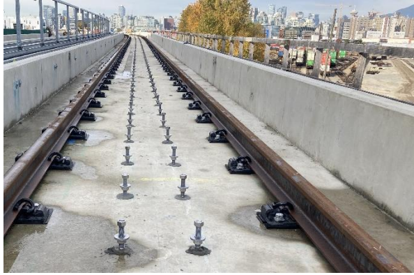
Figure 1: Elevated Guideway: Progressing with installation of the LIM (Linear Induction Motor) rail studs.
